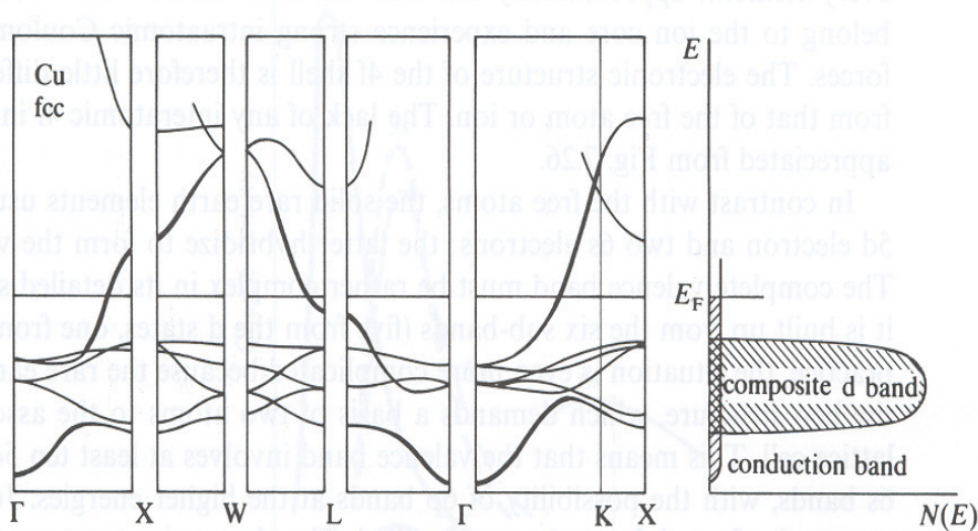
Figure 7.25 The complete band structure diagram for Cu along the major symmetry directions (compare with the Brillouin zone of Fig. 7.15b). The diagram to the right is a simple schematic representation of the integrated density of levels and is convenient as a basis for the discussion of many physical properties of the later 'd' metals. We shall soon find that the sp valence electrons are responsible for the electrical conductivity of these metals; one therefore speaks of the 'conduction band'. (After Segall 1962.)
