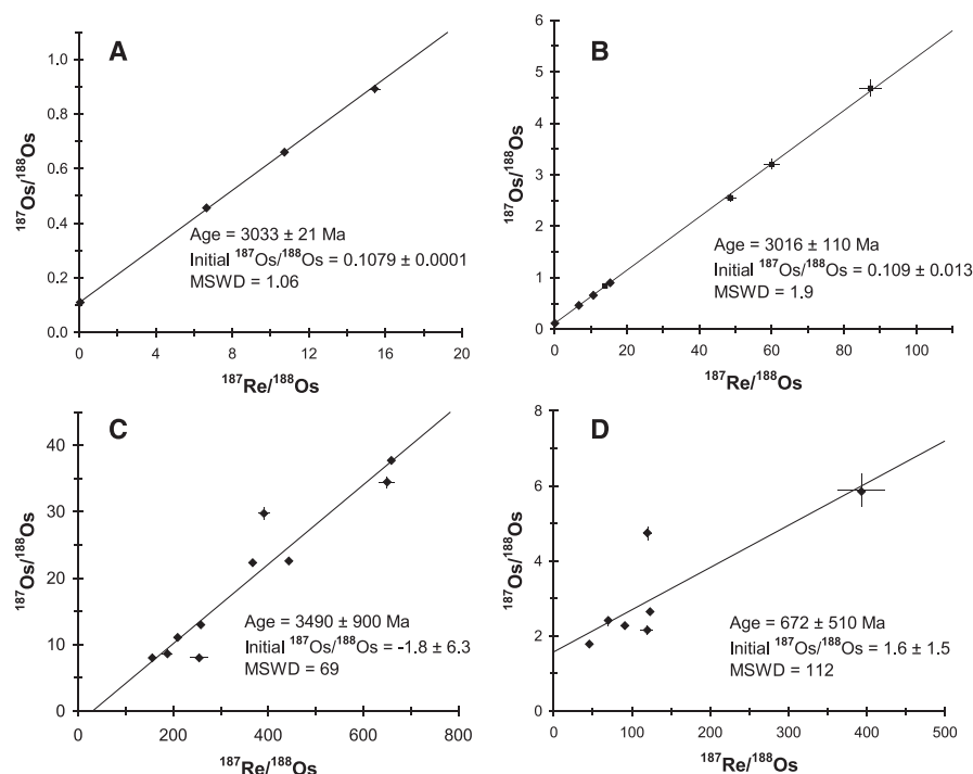
Fig. 1. Re-Os isochron diagrams for WSG samples. In all isochrons, errors are represented by crosses or are smaller than the symbols used. Errors were determined by using the greater of either the 2\sigma counting error ( 2SD/\sqrt{n} ) or by varying the Os blank between measured values of 1 to 2 pg. All isochrons were calculated using Isoplot (25). (A) VR gold samples. (B) VR gold and rounded VR pyrites. Filled squares represent pyrite samples; filled diamonds represent gold samples. (C) SR rounded pyrite samples. (D) VCR euhedral pyrites.
